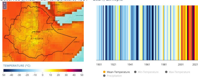
Figure 5 Observed average annual and monthly mean temperature of Ethiopia for 1901 - 2021 35
